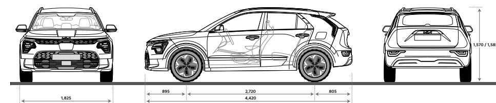
Dimensions EV (mm)
