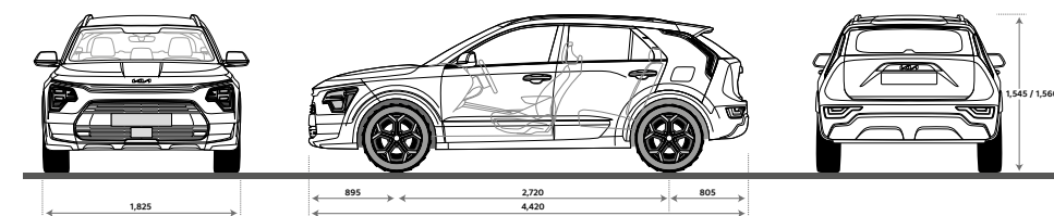
Dimensions HEV/PHEV (mm)
